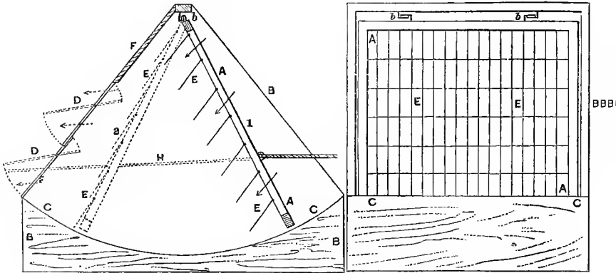
Fig. 13. Side view in section.
